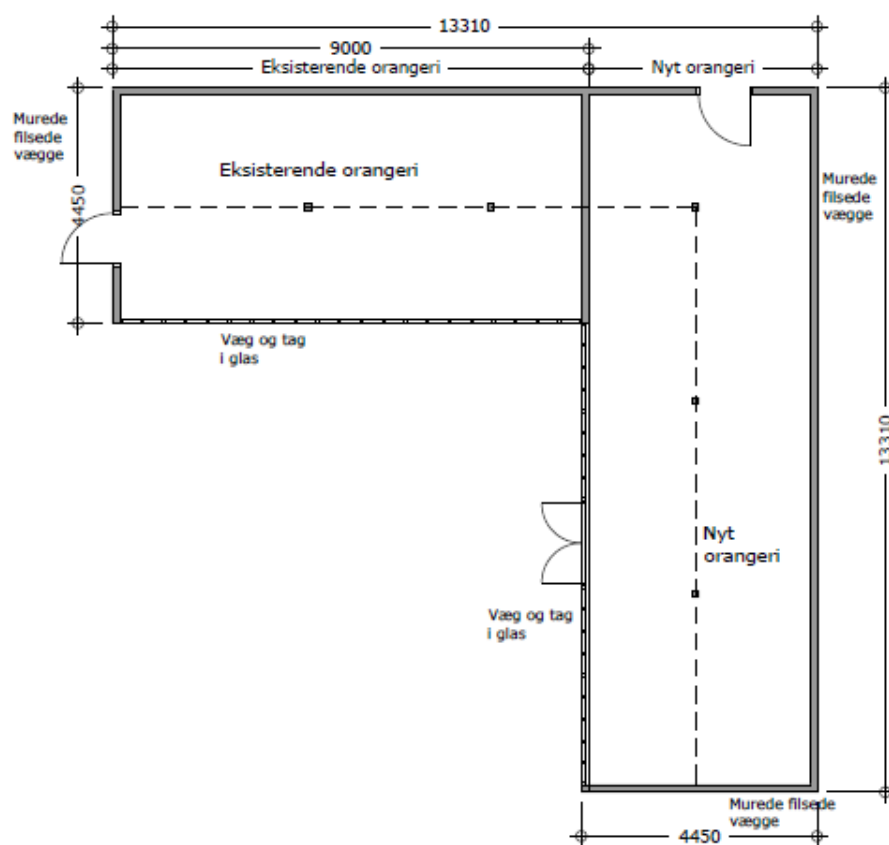
Figur 2. plantegning.
